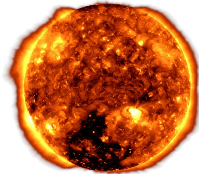
SDO/AIA 193 2021-04-15 05:58:29 UT 2021-04-15 05:58 SDO/AIA 193 (heq.bc)
