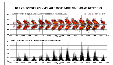
Butterfly diagram from Dr. David Hathaway, NASA MSFC ...
