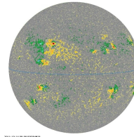
Average of magnetograms per Carrington rotation
