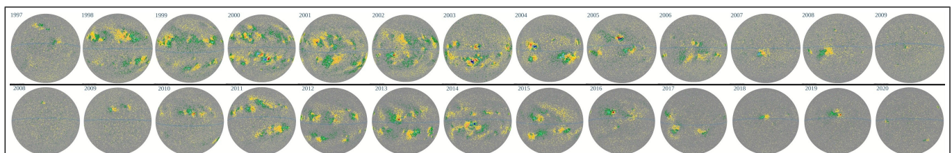
Magnetic field during SC 23 and 24, one image per year, selecting some more active time of that year. (SC23, SC24, video)
