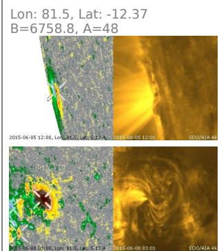
Sunspot since 2015-06-05 07:00, Mag since 2015-06-05 04:00 rolling from eastern limb, part of 150605_2000_19n_79_S13 this Box MaxMag=6758.8 MaxArea=48 (or cca 4000? on 2015-06-12 15:00)
