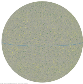
Example magnetogram of quiet Sun without sunspots
