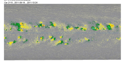
Average of magnetograms per Carrington rotation
