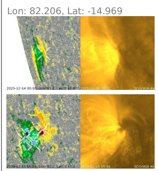
uncertain Sunspot since 2020-12-14 01:00 - it seems to have two negative sides which may be typical near-limb effect?, Mag since 2020-12-13 07:00 when rolled over limb
