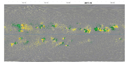
Magnetogram map for this date and interpolated far side between previous and following states
