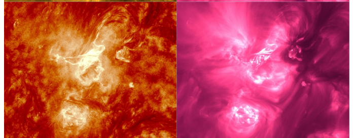
Detail of Sunspots on 2011-10-14 00:00
