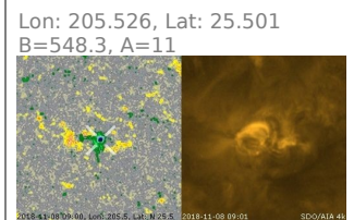
uncertain Sunspot since 2018-11-08 07:00 - looks like having two negative sides (it's -18 +15 -7 : the weaker right side was pre-existing there) but evolved into SC25 soon $w7, Mag since 2018-11-07 19:00, 181107_0800_1n_209_N21 MaxMag=548.3 MaxArea=11
