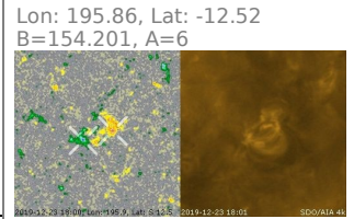
Sunspot since 2019-12-23 18:00 - too weak and not marked in Jpeg sources, Mag since 2019-12-23 09:00, 191223_1600_3_195_S11 MaxMag=154.201 MaxArea=6
