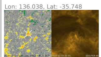
wrong Sunspot since 2020-12-16 19:00 with single polarity $w - in Fits sources already 2020-12-15 15:00, Mag since 2020-12-09 07:00 almost when rolled in
